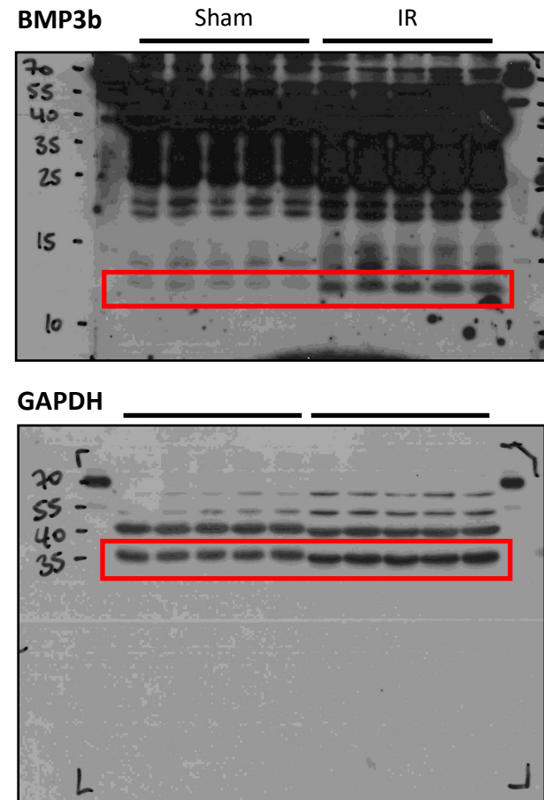
Full unedited gel for Figure 3
