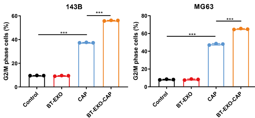
Figure S5. Statistics of the cell cycle at G2/M phase. *** P < 0.001 .
