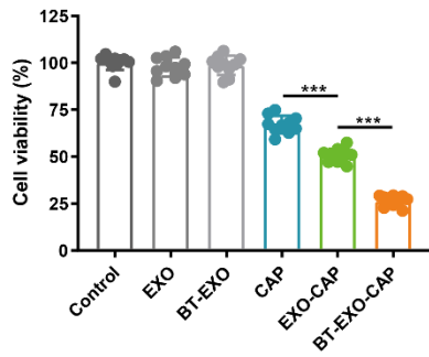
Figure S1. The effect of Exosomes, Bone targeting exosomes and Capreomycin on the activity of OS cells. *** P < 0.001 .
