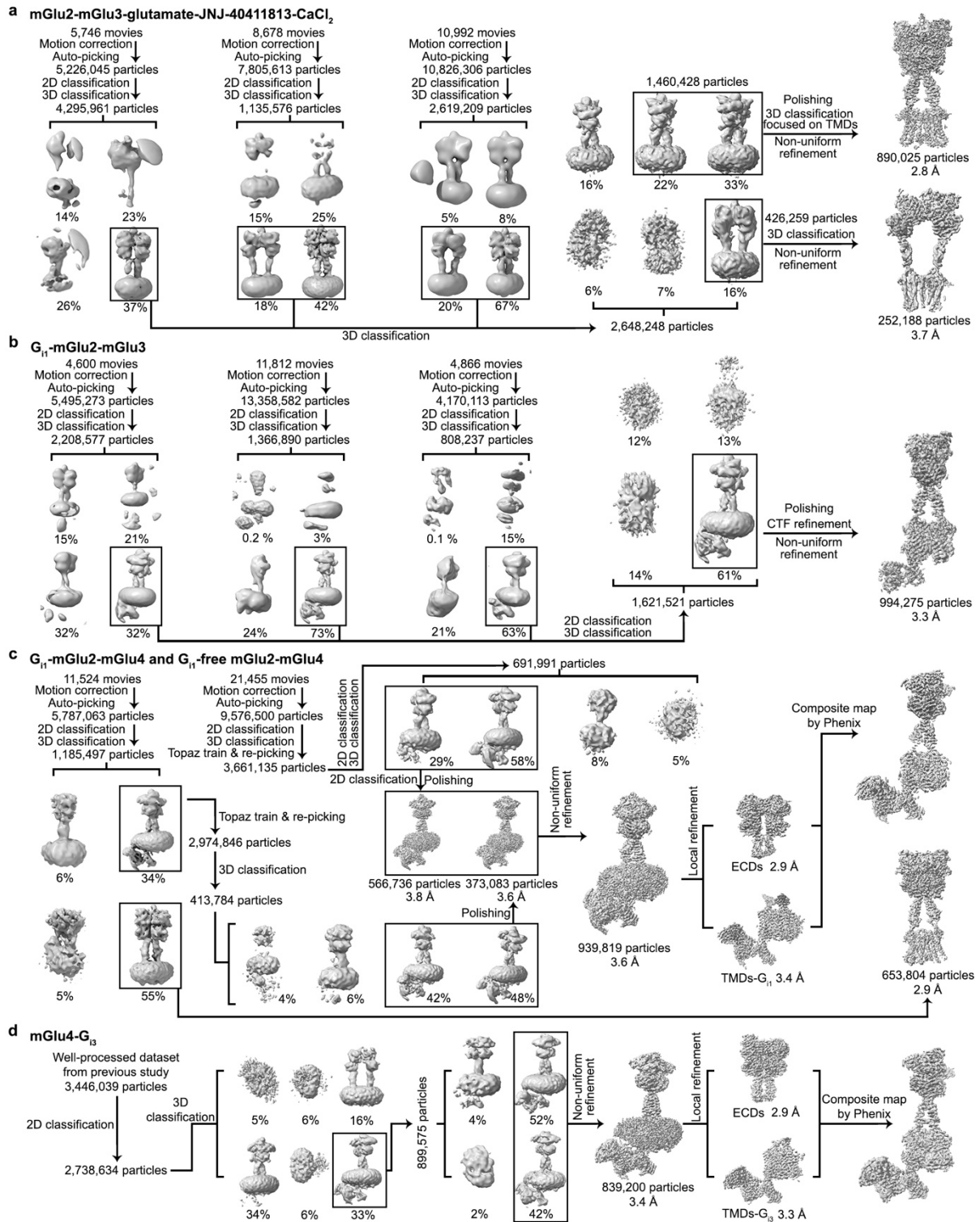
Fig. S3 Cryo-EM workflow of the agonist-bound mGlu2-mGlu3 and mGlu2-mGlu4 heterodimers and mGlu4 homodimer. a The mGlu2-mGlu3 heterodimer in the presence of glutamate, JNJ-40411813, and CaCl 2 . b The G i1 -bound mGlu2-mGlu3 heterodimer. c The G i1 -bound and G i1 -free mGlu2-mGlu4 heterodimers. d The G i3 -bound mGlu4 homodimer.
