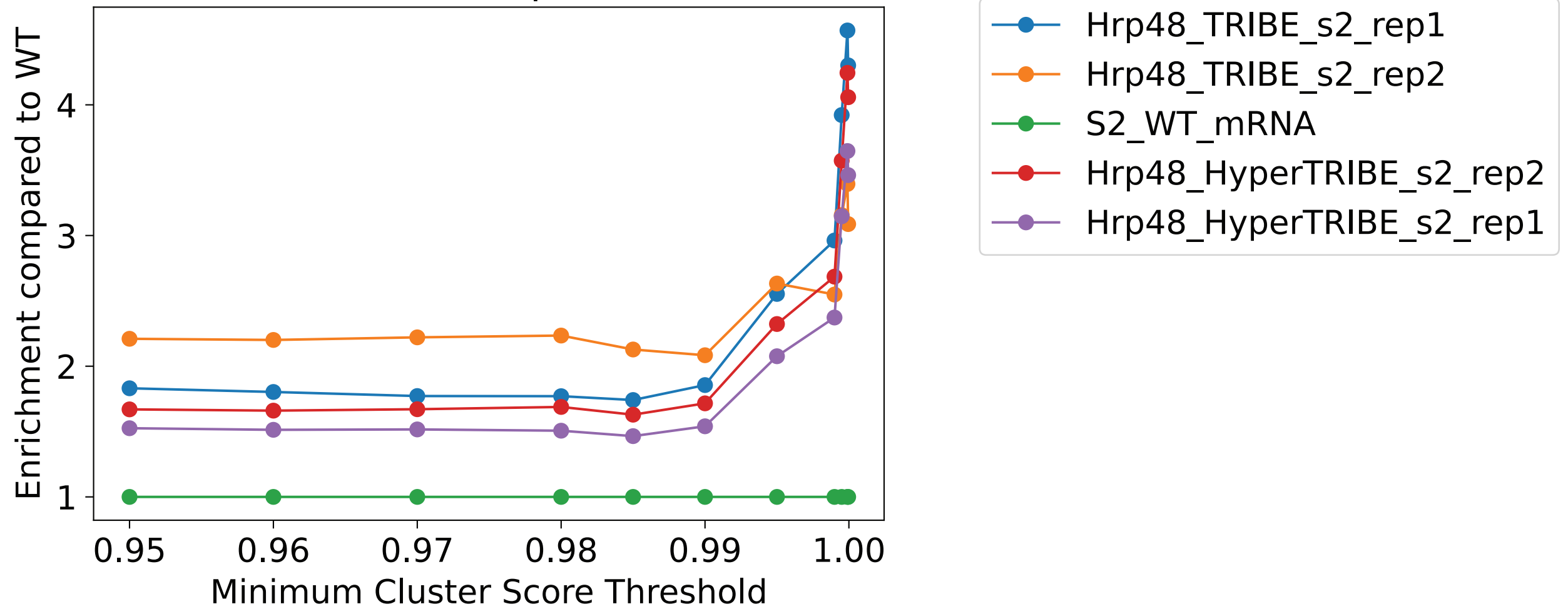
Fraction of FLARE clusters overlapping fusion eCLIP: Enrichment compared to WT
