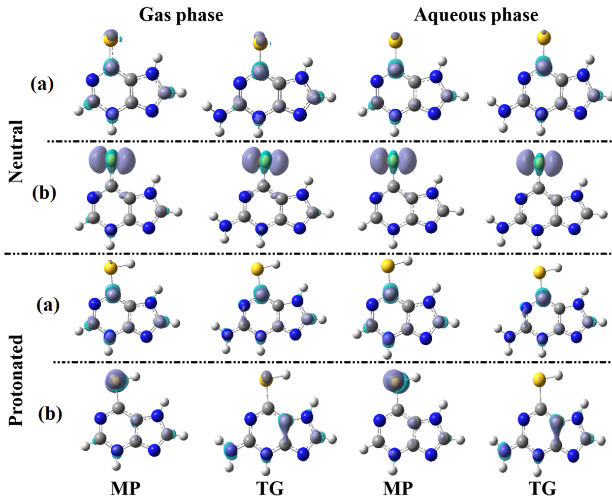
Figure S1. Plots of (a) nucleophilic ( f_k^+(r) ) and (b) electrophilic ( f_k^-(r) ) Fukui function indices isosurfaces of the 6-Mercaptopurine (MP) and 6-Thioguanine (TG) drugs.
