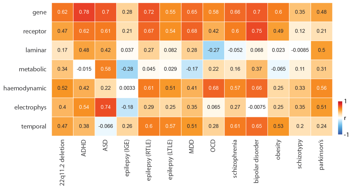
Figure S9. Contributions of connectivity modes to disease vulnerability | We repeat the procedure in Fig. 4 after regressing the exponential relationship with Euclidean distance (shown in Fig. 1b) from each connectivity mode. The data underlying this figure can be found at https://github.com/netneurolab/hansen_many_networks .
