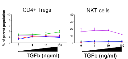
Fig. S3: Expression of TGFβ-decoy receptor does not affect primary T cell marker expression for stimulation, exhaustion or differentiation in the presence of different concentrations of TGFβ. A) Line graphs representing the expression of CD69 as a marker for T cell stimulation, B) PD1 as a marker for exhaustion, and C) CD57 and D) KLRG1 as marker for T cell differentiation. E) the ratio of CD4+ T cells is not affected whereas the proliferation of NKT cells seems slightly enhanced in cells expressing HA-GPI-ecto-TβRII. Line graphs display the mean and SEM of at least 6 biological replicates.
