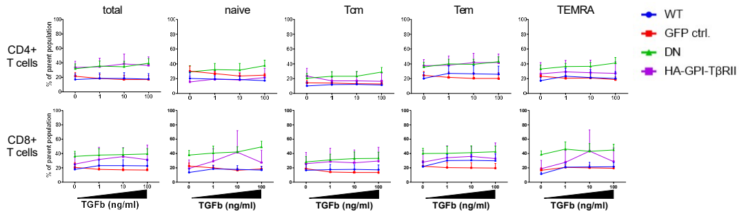
Fig. S3: HA-GPI-ecto-TGFβRII has no effect on stimulation or exhaustion or the expression of the chosen marker for differentiation in ATCs in the presence of recombinant TGFβ
