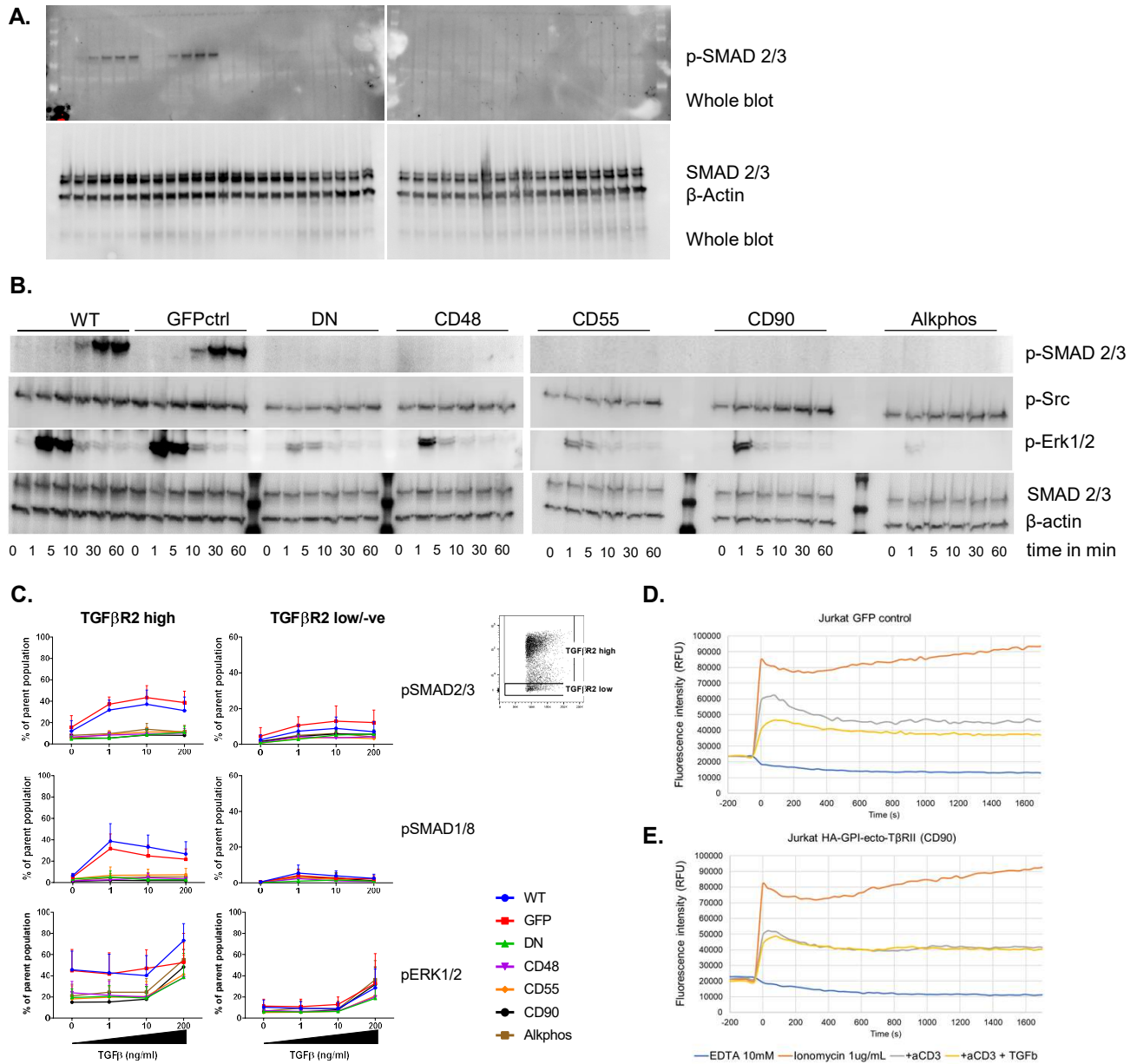
Fig. S1: A) Whole WB of pSMAD2/3 from Fig. 2. B) WB of strongly inhibited TGF \beta -dependent SMAD and ERK signalling in Jurkat cells expressing TGF \beta -decoy receptors. No changes in Src signalling was observed. C) Flow cytometric analysis of p-SMAD2/3 and 1/8 and ERK1/2 in Jurkat cells gated for either high or low expression of TGF \beta R2 (decoy or WT). D+E) Readings of calcium flux in the presence of TGF \beta in either stimulated GFP-ctrl. or HA-GPI-ecto-T \beta RII expressing Jurkat cells.
