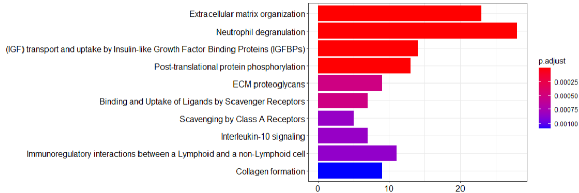
PC1 top 250 contributors
