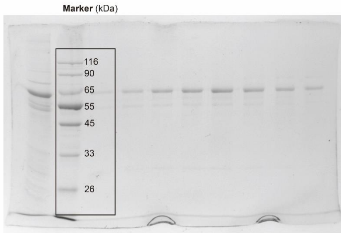
Uncropped SDS-PAGE gel for the E232Q mutant of AtABCG25 . Related to Extended Data Fig. 8a.
