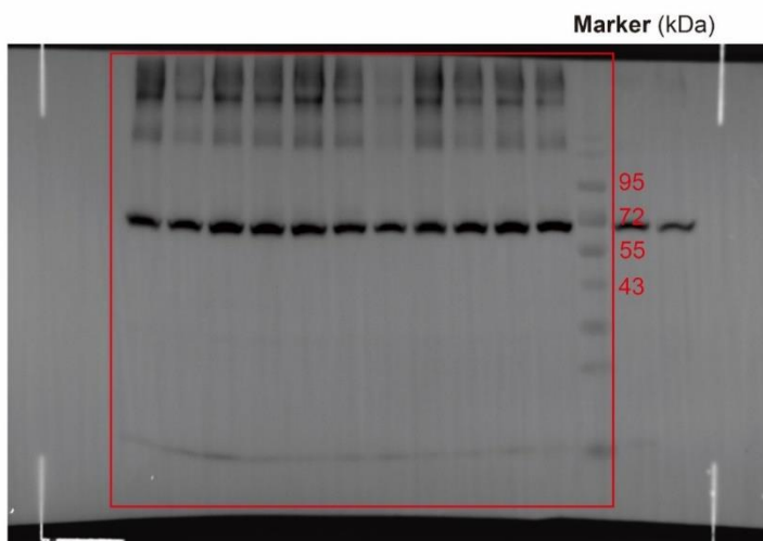
Uncropped Western blot of AtABCG25 variants using anti-Flag antibody. Related to Extended Data Fig. 5i.
