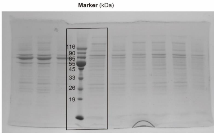
Uncropped SDS-PAGE gel for the WT AtABCG25 purified with DDM extraction. Related to Extended Data Fig. 6e.
