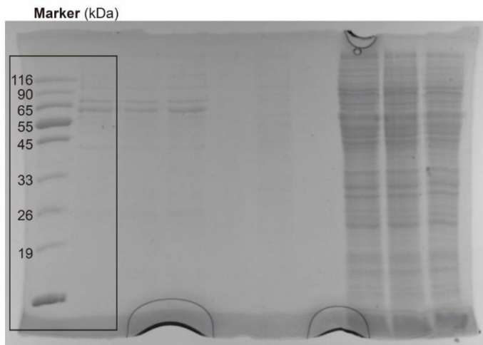
Uncropped SDS-PAGE gel for the WT AtABCG25 purified with DDM extraction and ABA-added during the whole purification steps. Related to Extended Data Fig. 6h.
