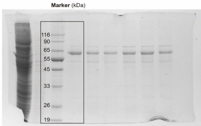
Uncropped SDS-PAGE gel for the WT AtABCG25 purified with DDM plus CHS extraction. Related to Extended Data Fig. 3a.
