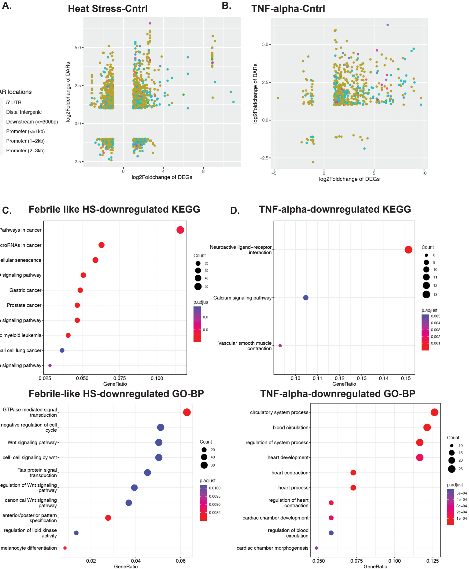
Figure S3. Related to Fig.3. ATAC-seq and RNA-seq integrative analysis. A. Genomic features of ATAC-seq and RNA-seq in HS-C samples. B. Same as A but in T-C samples. C. KEGG and GO-BP analysis of downregulated pathways in HS-C samples. D. Same as C but in T-C samples.
