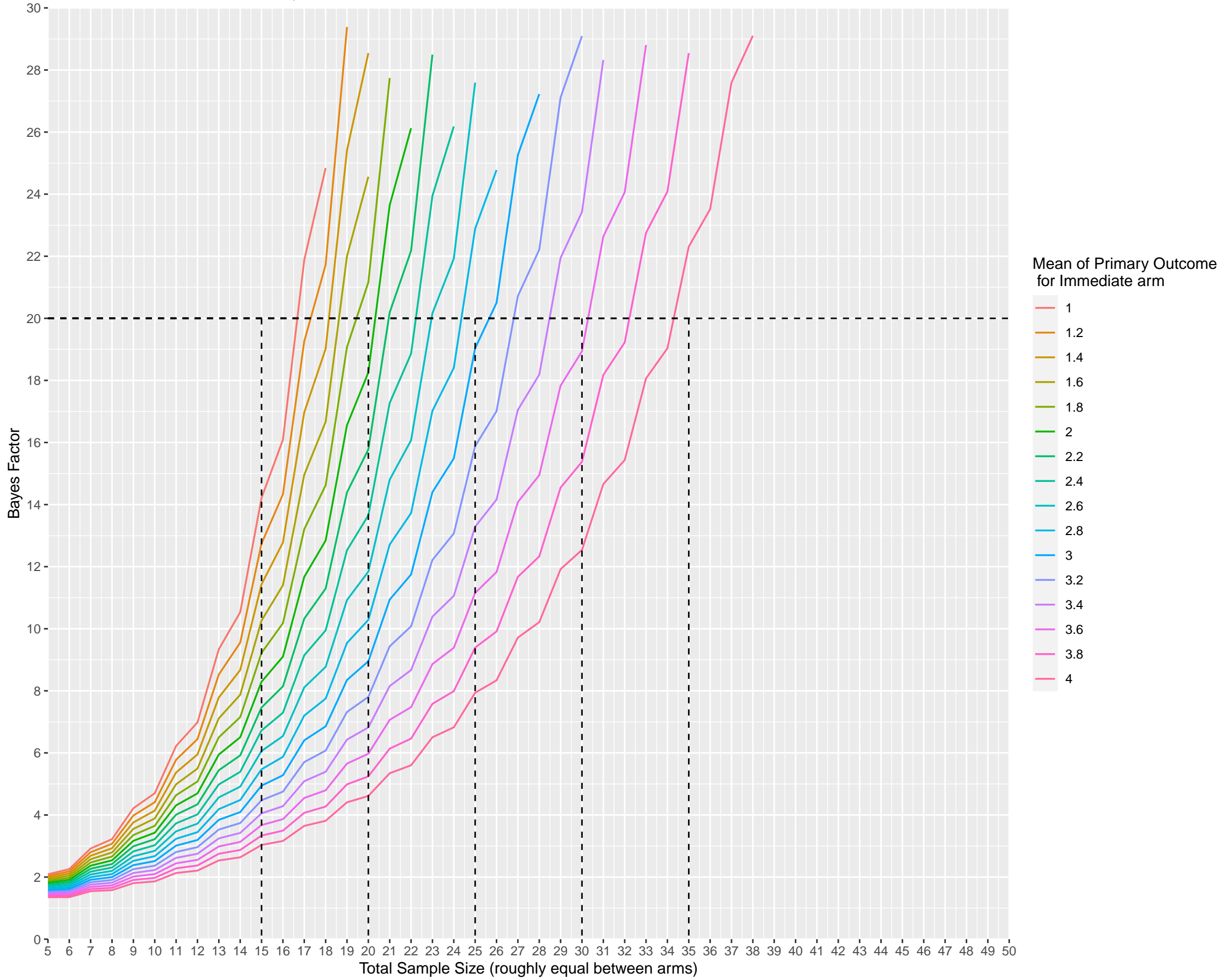
Bayes Factor vs Sample Size: Testing for Superiority of immediate arm vs delayed arm
