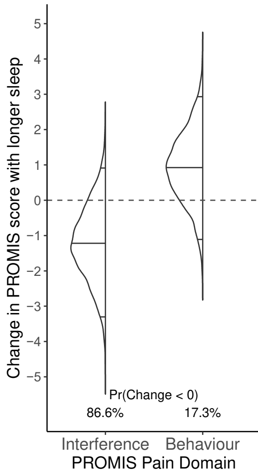
Appendix Figure 1. Posterior density plots (rotated 90 degrees) for PROMIS Pain Interference and Pain Behaviour. Please see figure 3c for a description of posterior density plots.
