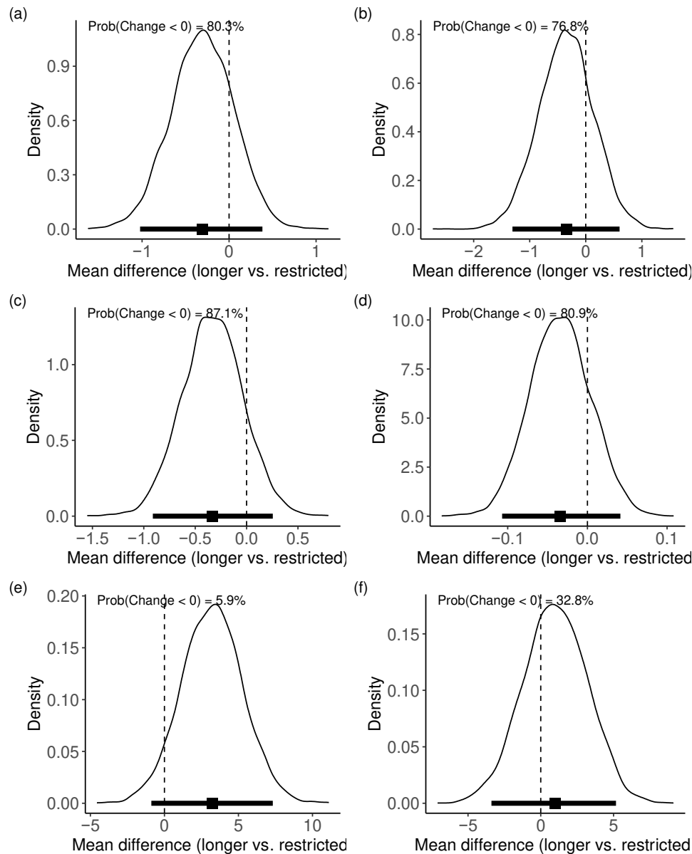
Appendix Figure 2. Posterior density plots for (a) active joint count, (b) physician global assessment of disease activity, (c) patient global assessment of disease activity, (d) CHAQ score, (e) quality of life (QoL) score, (f) HRQoL score. These outcomes are all on a different scale, so are shown on different plots. Please see figure 3c for a description of posterior density plots.
