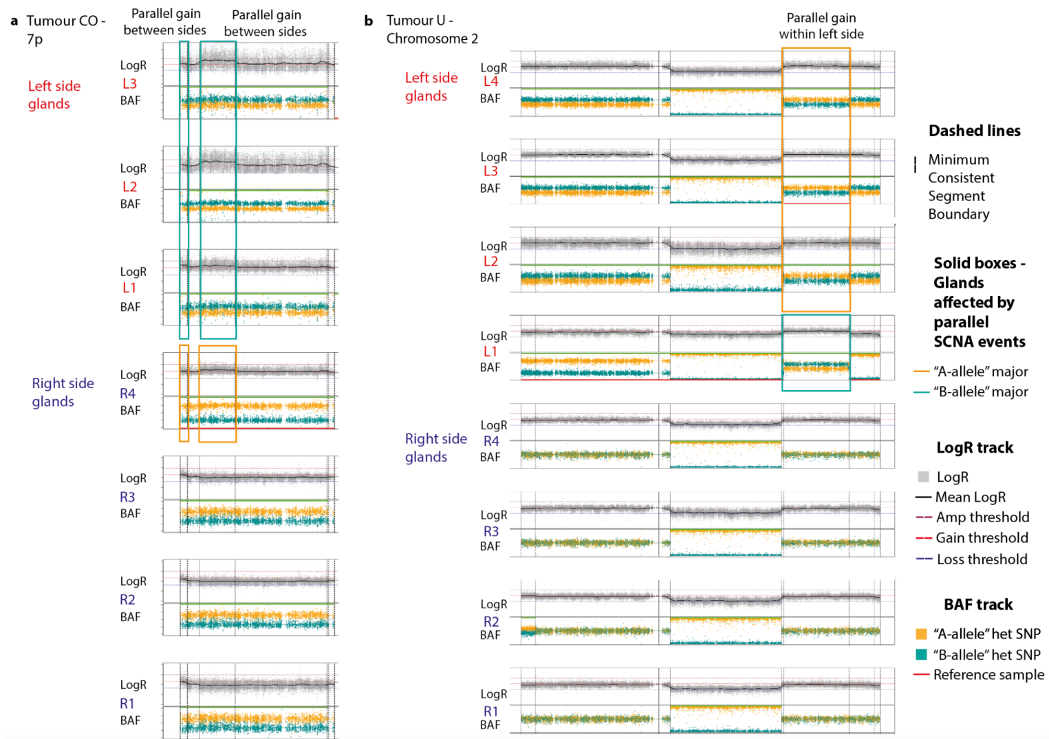
Supplementary Figure 7: Examples of parallel SCNA events in the Sottoriva et al [1] colorectal adenocarcinoma cohort. a) Examples of parallel gain events on chromosome arm 7p, observed between glands on different sides of the tumour. b) Example of a parallel gain event on chromosome 2, observed within glands on the same side of the tumour. Tumour IDs shown match those in the original publication [1].
