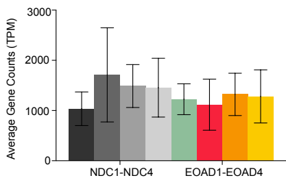
D Average Expression of Neural Progenitor Cell Type Markers
