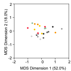
H Neural Progenitor Cell Type Markers
