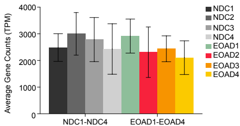
E Average Expression of Oligodendrocyte Cell Type Markers
