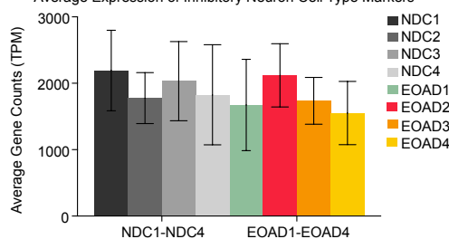
G Average Expression of Inhibitory Neuron Cell Type Markers
