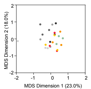
I Oligodendrocytes Cell Type Markers
