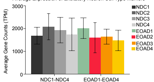
F Average Expression of Excitatory Neuron Cell Type Markers
