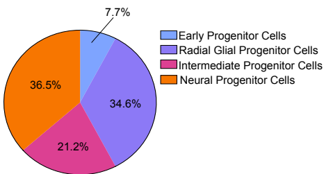
D Average Expression of Neural Progenitor Cell Type Markers
