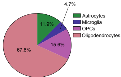
E Average Expression of Oligodendrocyte Cell Type Markers
