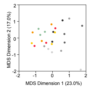
K Inhibitory Neuron Cell Type Markers
