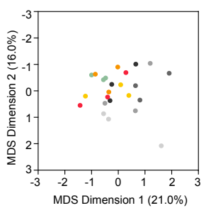
J Excitatory Neuron Cell Type Markers
