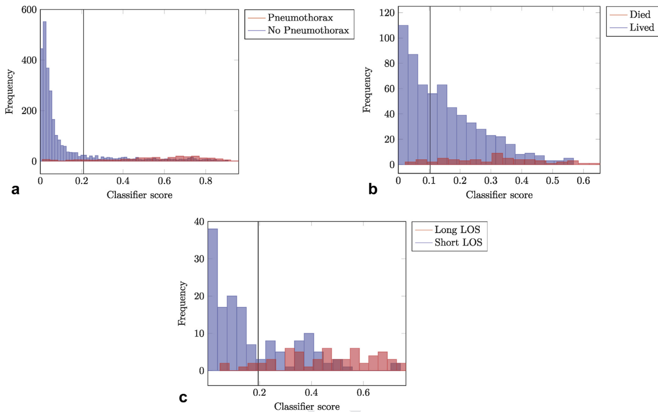
Figure E1. (a–c) Probability histograms. The positive class (class of interest) is plotted in red, and the negative class is plotted in blue. The vertical black line indicates the probability threshold corresponding to 90% sensitivity. (a) TTB probability histogram. (b) TIPS probability histogram. (c) UAE probability histogram.
