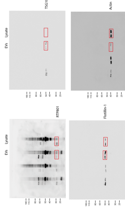
Figure S2
