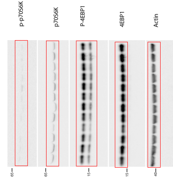
Figure S10
