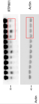
Figure S9
