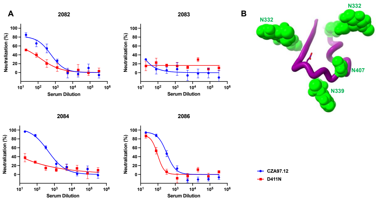
S3 Figure. The mapping of autologous NAb epitopes in sera from rabbits immunized with CZA97.012 SOSIP.664. A. The immunization sequence (70) and the D411N mutant have been described (69). Neutralization of CZA97.012 parental and D411N-mutant PV by rabbit sera was analyzed. The diagrams show a sigmoid curve fitted to % neutralization as a function of the serum dilution factor. The data points are means of 5-11 replicates \pm s.e.m. B. A cryo-EM model of the CZA97.012 SOSIP.664 V4- \beta 19 transition (backbone in purple) is shown with N-linked glycans near D411 (side-chain as red stick) depicted with carbohydrate residues as green spheres.
