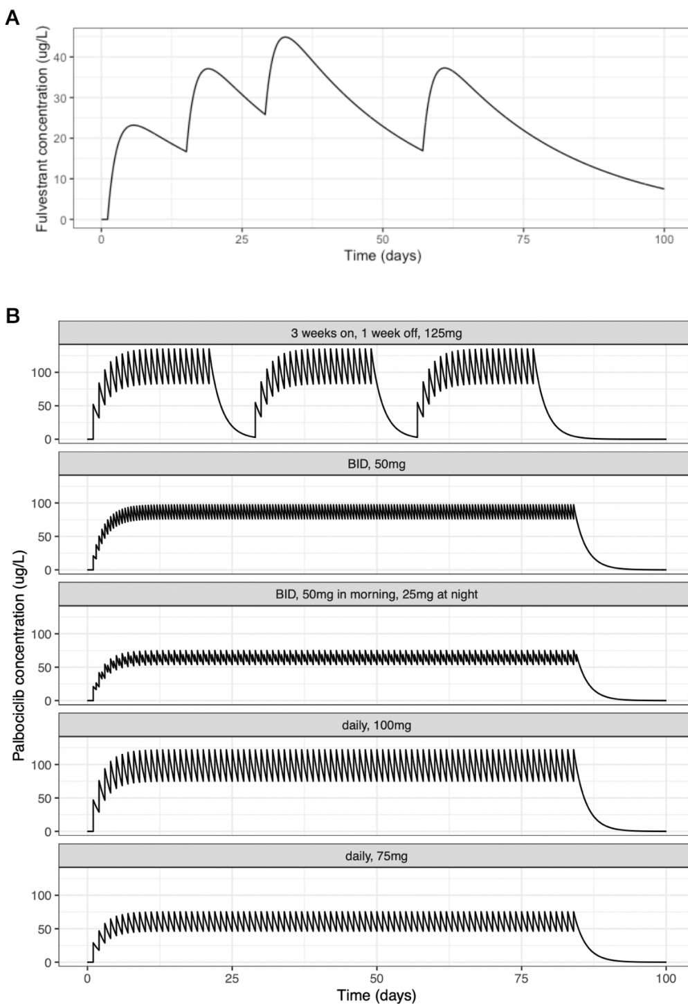
Fig. S9 In silico trial predictions of multiple palbociclib treatment administration schedules in combination with fulvestrant. Each panel represents the plasma concentration of (A) fulvestrant and (B) palbociclib for each treatments schedule given by the table.
