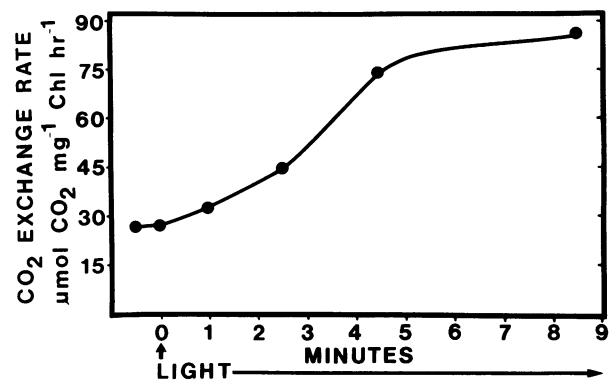
FIG. 3. Time course of net CO 2 uptake during the transition from the dark to the light at 2,500 μl CO 2 l -1 and 1,000 μE m -2 s -1 .
