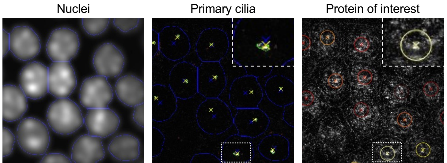
Figure S7. Overview of the outcome of the MATLAB script-based analysis. Nuclei segmentation (left) and primary cilia segmentation (middle) defined as the brightest 3D objects overlapping a nucleus region. Primary cilium bases (yellow cross) are identified as the closest cilium voxel to the centroid of the corresponding nucleus region.
