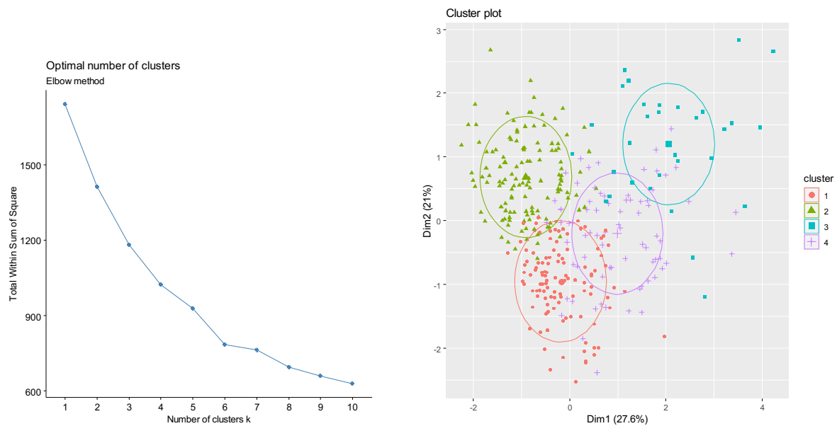
Supplementary Figure 1. Elbow plot and visualization of Clusters
