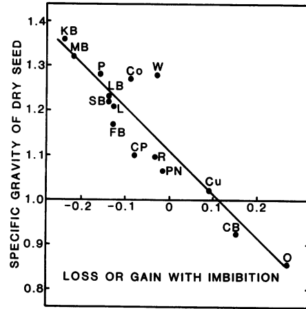
FIG. 2. The specific gravity of dry seeds of 15 species, and its relationship to loss or gain of specific gravity during imbibition. Slope = -0.077 , R = -0.923 . KB = kidneybean; MB = mungbean (Blackeye); P = Alaska pea; W = wheat (Little Club); Co = corn (Merit); LB = limabean (Fordhook); SB = soybean (Cutler); L = lettuce (Grand Rapids); FB = favabean; CP = cowpea (California Buckeye); R = radish; PN = peanut; Cu = cucumber (Straight Eight); CB = castorbean; O = oat (Astro).
