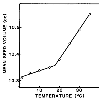
FIG. 5. Equilibration of fully imbibed soybeans at various temperatures (2 to 35°C) results in changes in the seed volume. Average of 12 experiments, each of which started with 5 g dry soybeans.
