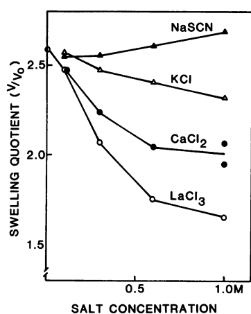
FIG. 4. Effects of various salts on the swelling quotient of soybean seeds. All data are for 24-h imbibition.
