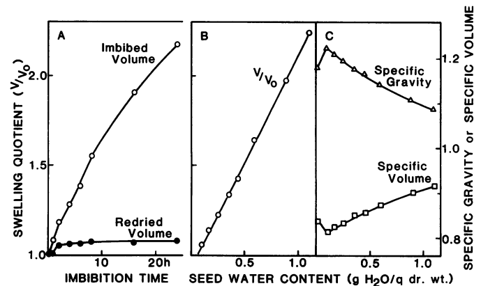
FIG. 3. Relationship between water content and soybean seed volume. A, Changes in the swelling quotient when the seeds are allowed to imbibe free water for differing periods of time, and the degree of recovery of original volume when the seeds were subsequently redried to air dryness. B, The relationship between the swelling quotient and the seed water content. C, Calculated specific gravity and specific volume in relation to seed water content. All data are from the same experiment.
