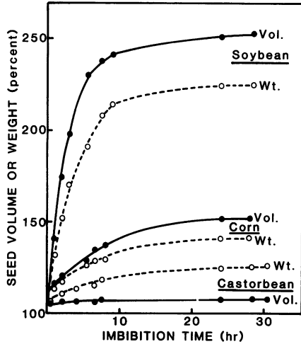
FIG. 1. Representative time course plots for volume and weight gains during imbibition of soybean, corn, and castorbean seeds.
