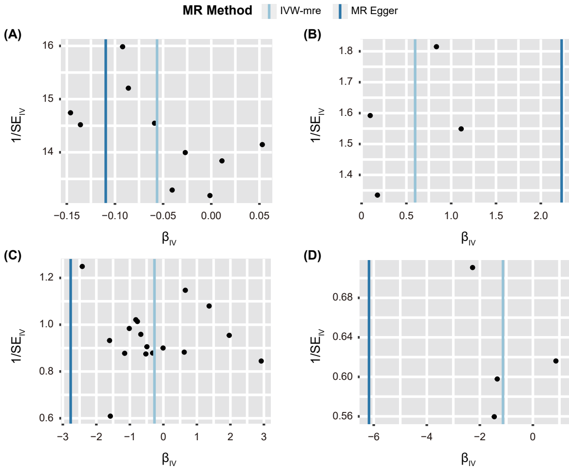
Figure S1: Funnel plots of the genetic associations between PA and LBP. (A) accelerometer-based PA (average acceleration); (B) accelerometer-based PA (acceleration fraction > 425 milligrams); (C) self-reported moderate-to-vigorous PA; (D) self-reported vigorous PA. The light blue line represents the IVW estimate, and the dark blue line represents the MR - Egger estimate. IVW-mre, multiplicative random effects inverse variance weighting.
