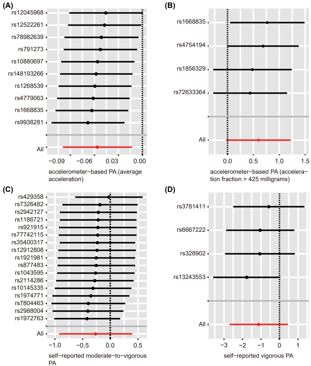
Figure S4: Leave-one-out sensitivity analysis of single SNP for LBP. (A) accelerometer-based PA (average acceleration); (B) accelerometer-based PA (acceleration fraction > 425 milligrams); (C) self-reported moderate-to-vigorous PA; (D) self-reported vigorous PA. Leave-one-out sensitivity analysis is performed to ascertain if a single SNP disproportionately influences an association for LBP. Each black point in the forest plot represents the MR analysis (using IVW) excluding that particular SNP. The overall analysis, including all SNPs, is also shown for comparison..
