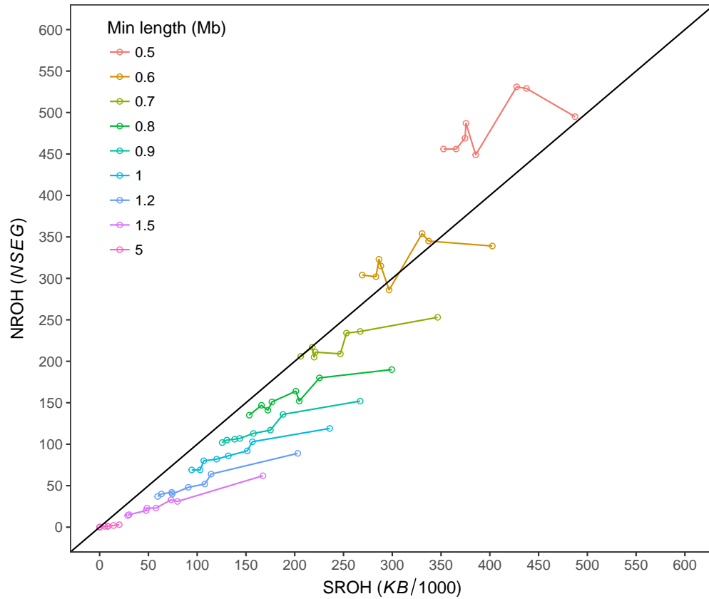
Figure S10.1: Plot of the number of runs of homozygosity NROH ( NSEQ ) against the total length of runs SROH ( KB/1000 ) in the PLINK report for a subset 0.5 – 5Mb of the variable minimum ROH lengths. At 0.6Mb minimum length the population seems bottlenecked with most points close to or at the diagonal. Above 0.6Mb the population seems bottlenecked and consanguineous with the points below and right shifted from the diagonal. At 1.5Mb the points left shift towards the diagonal, and at 5Mb the leftmost point is back near the diagonal.
