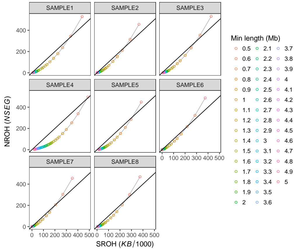
Figure S10.2: Plots of the number of runs of homozygosity NROH ( NSEQ ) against the total length of runs SROH ( KB/1000 ) in the PLINK report for the minimum lengths of ROH > 0.5Mb. At about 1.0Mb the points are maximum shifted to the right from the diagonal.
