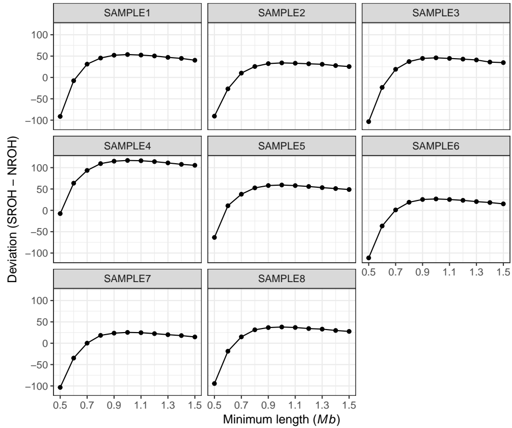
Figure S10.3: Plots of deviation SROH (KB/1000) - NROH (NSEQ) from the linear diagonal in the NROH versus SROH plots shown for minimum ROH lengths between 0.5 and 1.5Mb. For all the samples the SROH is below the diagonal (deviation > 0 ) for minimum ROH lengths above 0.7 – 0.8Mb and the maximum deviation is found at 1.0Mb.
