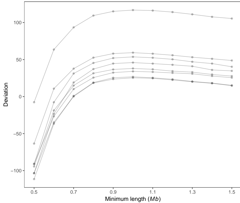
Figure S10.7: Plot of deviation SROH (KB/1000) - NROH (NSEQ) from the linear diagonal in the NROH versus SROH plots shown for minimum ROH lengths between 0.5 and 1.5Mb. For all the samples the SROH is clearly below the diagonal (deviation > 0 ) for minimum ROH lengths above 0.7 – 0.8Mb and the maximum deviation is found at 1.0Mb.
