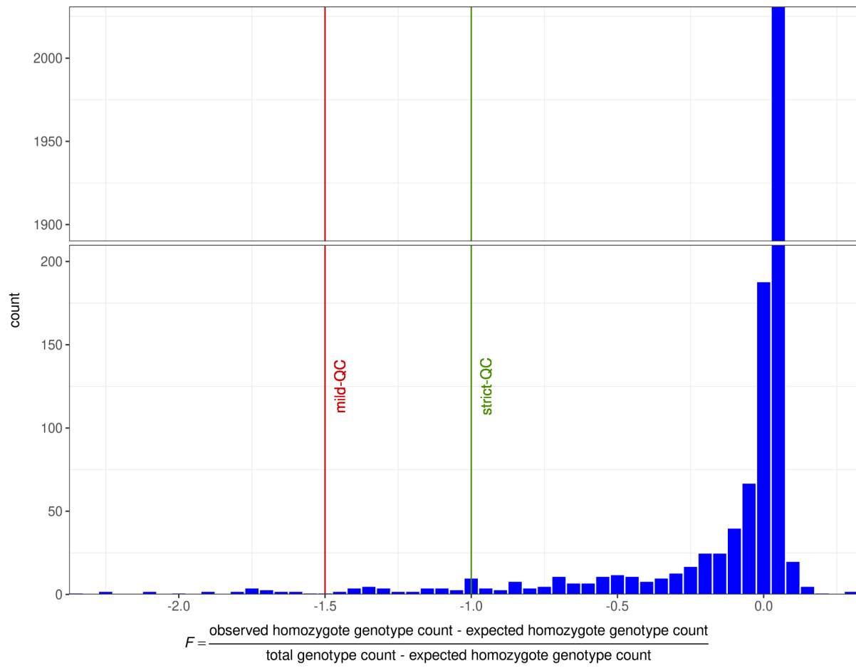
S5 Fig. Homozygosity / Heterozygosity outliers
