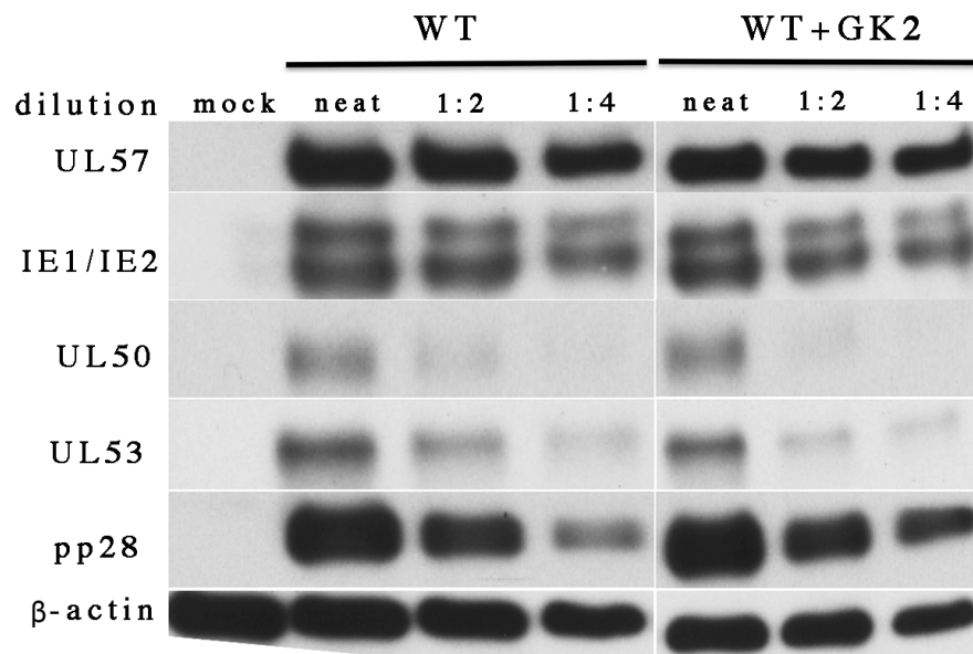
S4 Fig. Effect of GK2 on HCMV protein expression in infected cells. HFF cells were mock infected or infected with WT HCMV at an MOI of 1. Following absorption, medium containing either DMSO or 10 \mu M GK2 was added. At 72 hpi, cells were lysed, proteins resolved using SDS-PAGE, and the expression of the viral proteins indicated to the left was assessed by immunoblotting. Similar results were obtained in a second independent experiment.
