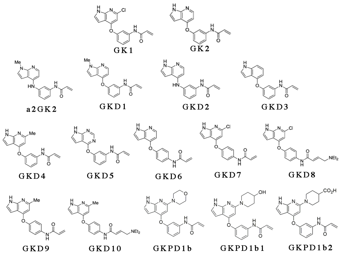
S6 Fig. The chemical structures of analogs of GK1 and GK2
