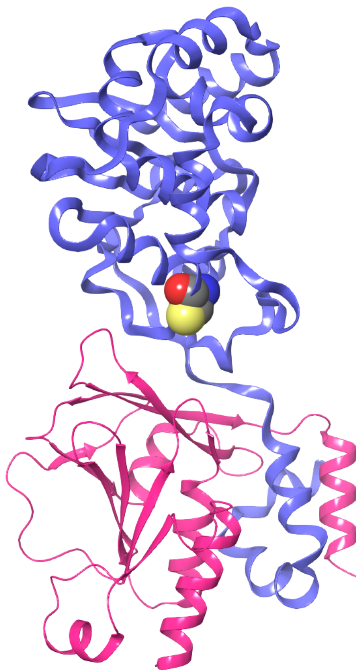
S9 Fig. Location of Cys214 relative to the subunit interfaces of the HCMV NEC. UL53 is shown in blue and UL50 in red with Cys214 shown in a space filling model just above the “B” interface of the NEC. The “A” interface involving segments of UL53 within the “vise” of UL50 is below and to the right of Cys214.
