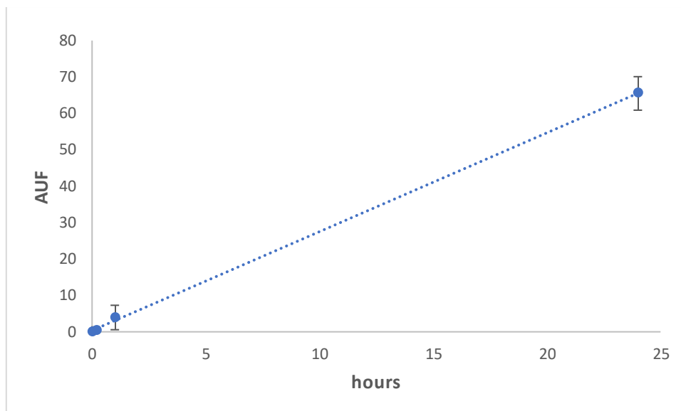
Additional file 2. Oligomerization of A \beta 42 peptide after dilution to PBS buffer at 4°C for 24 hours, measured by arbitrary units of fluorescence (AUF) after staining with Thioflavin-T.
