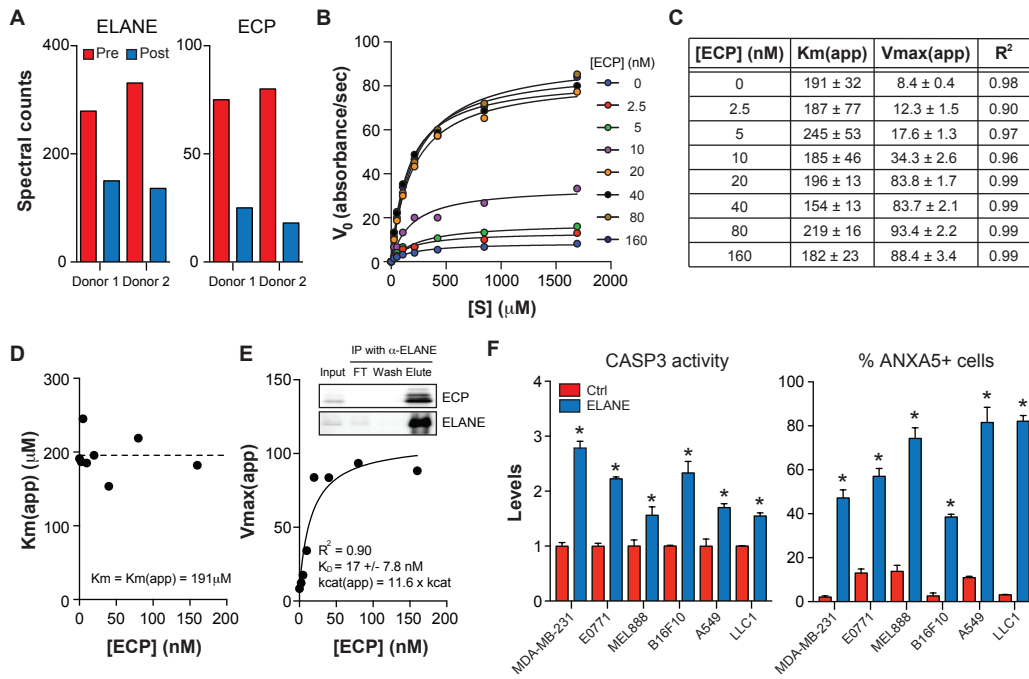
Figure S2. ECP is a type II allosteric activator of ELANE, related to Figure 2
