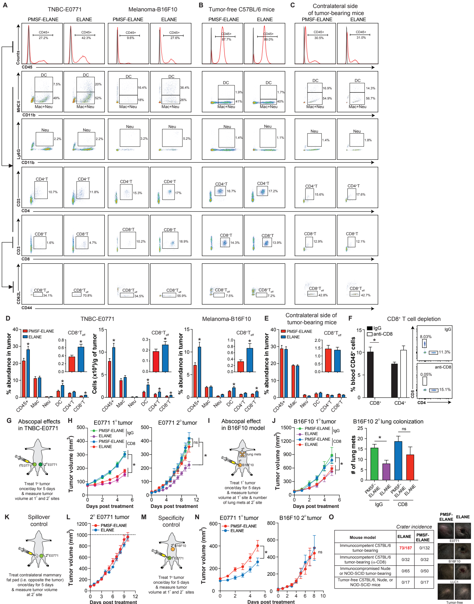
Figure S6. ELANE induces a CD8 + T-cell-mediated abscopal effect in syngeneic models, related to Figure 6
