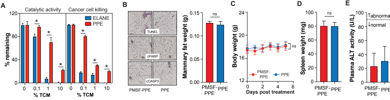
Figure S7. PPE exhibits minimal toxicity in tumor-free mice, related to Figure 7
