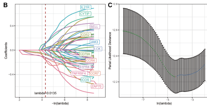
Supplementary Figure 1. Establishment of a prognostic signature. (A) Univariate Cox regression analysis of genes correlated with HNSC prognosis. (B, C) LASSO analysis for significant genes associated with HNSC prognosis.
