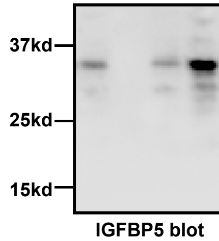
Figure 6F
