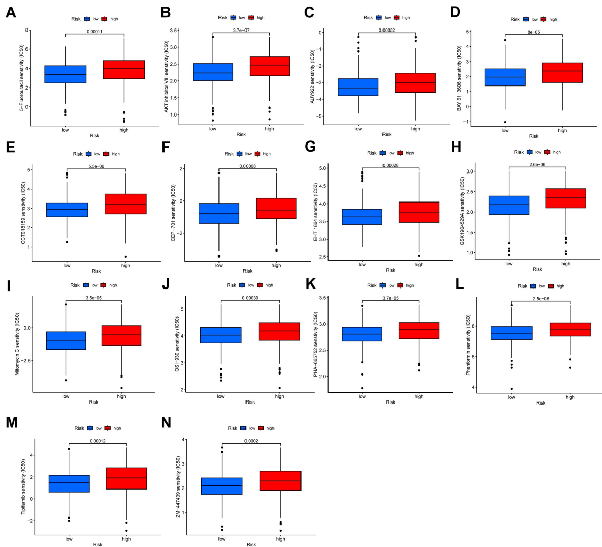
Supplementary Fig. S1 Drug susceptibility analysis. (A–N) Fourteen drugs demonstrated lower IC50 values for patients in the low-risk group
