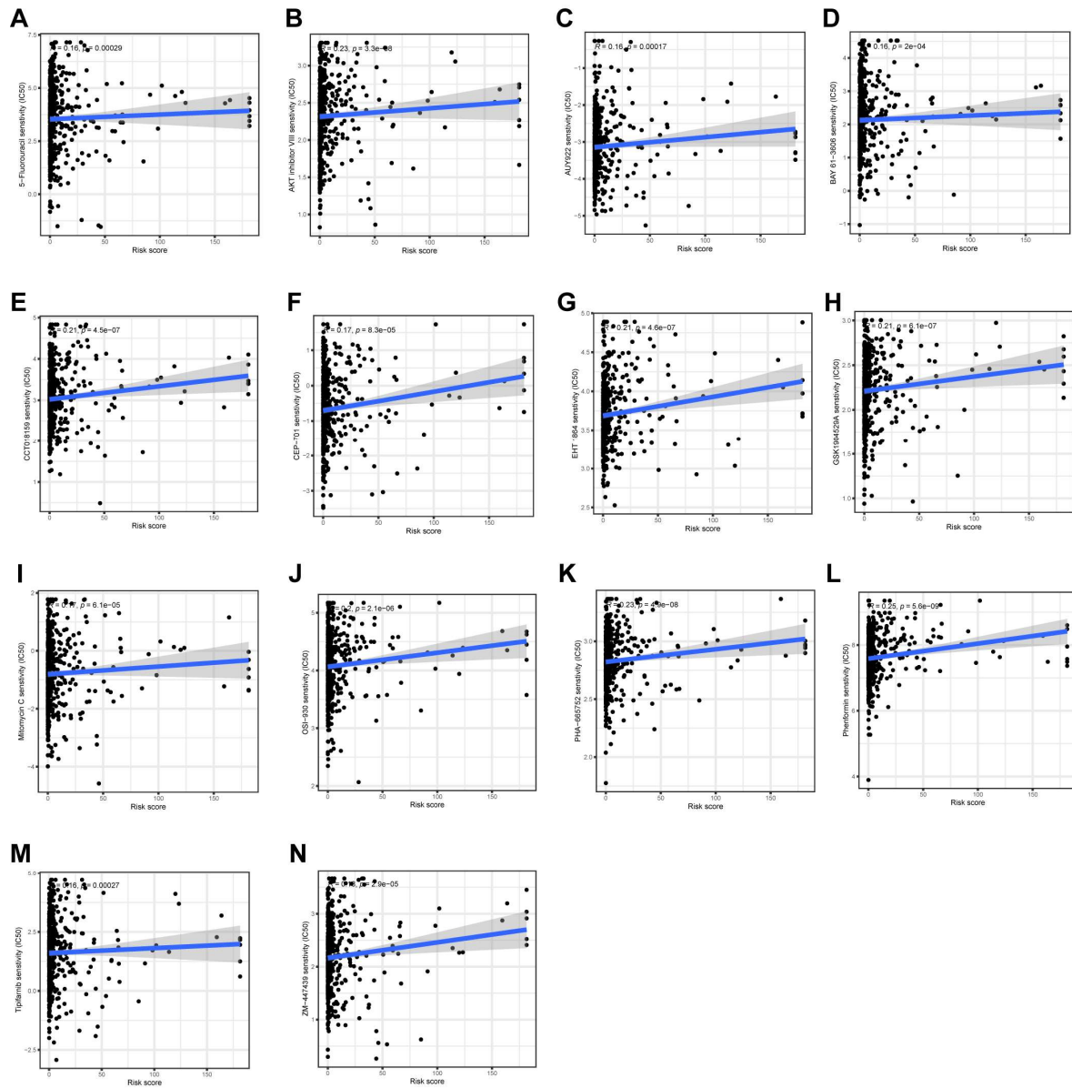
Supplementary Fig. S2 Drug susceptibility analysis. (A–N) The correlation between the IC 50 values and risk scores of the fourteen aforementioned drugs
