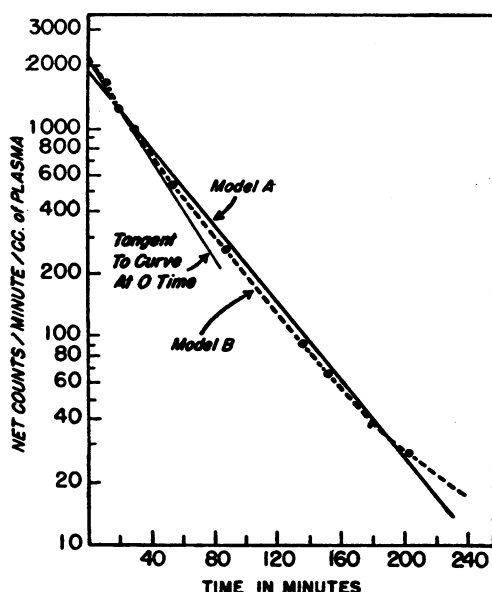
FIG. 1. GRAPHIC PRESENTATION OF THE TWO MODELS USED FOR COMPUTATION OF THE RATE OF REMOVAL OF RADIOIRON FROM THE PLASMA
