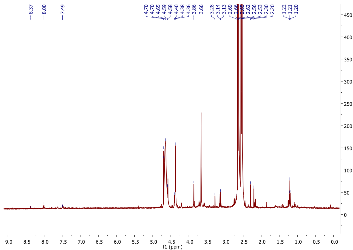
Figure S3. ^1\text{H-NMR} spectra of gold nanoparticles conjugated with NG-ssDNA 11 .
