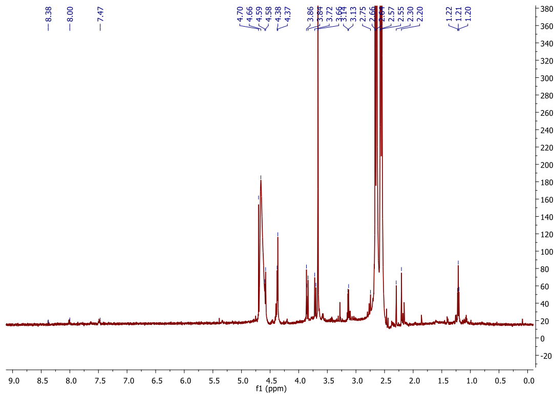
Figure S2. ^1\text{H-NMR} spectra of gold nanoparticles conjugated with CT-ssDNA 1 .
