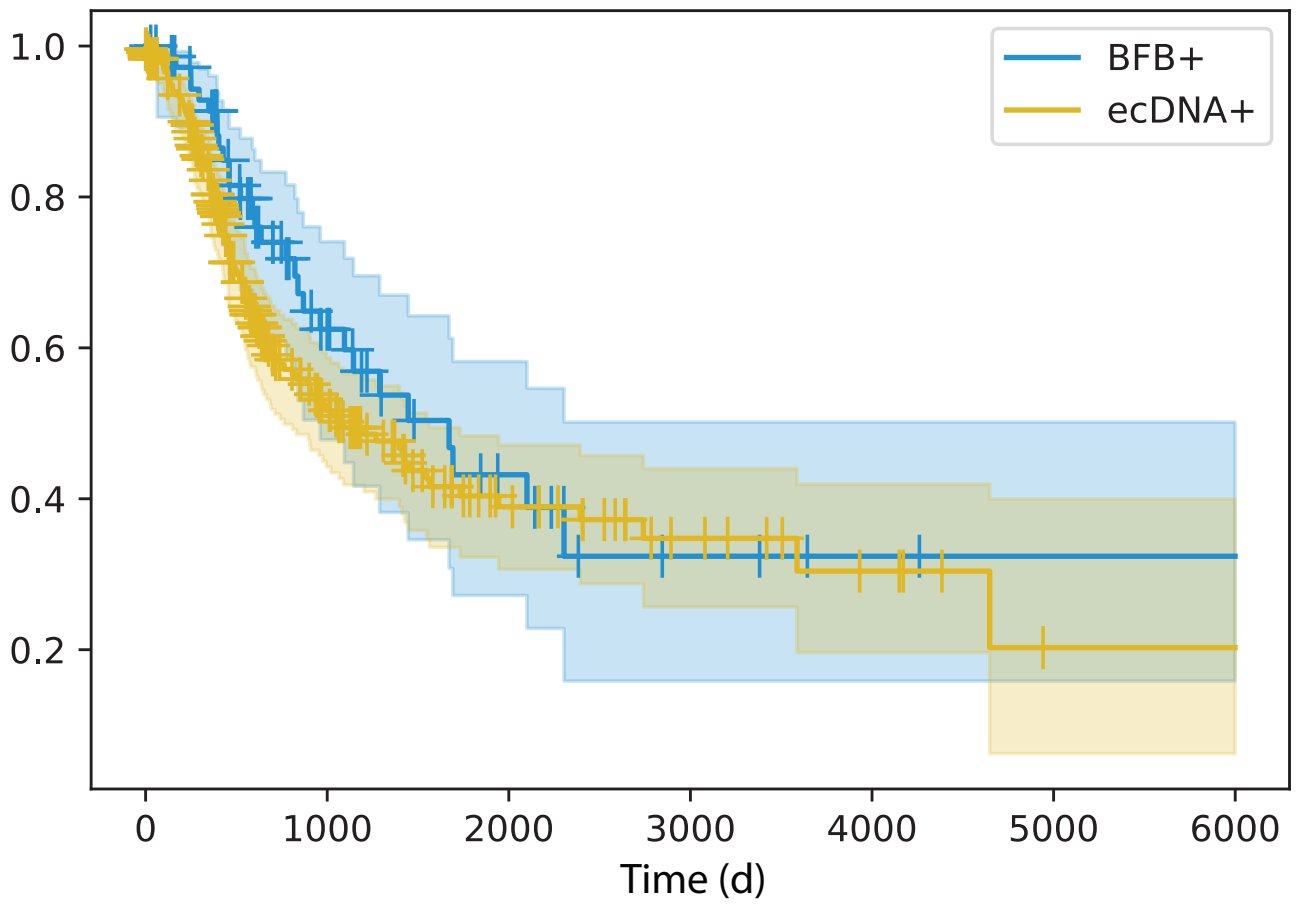
Survival and ecDNA/BFB status in TCGA
