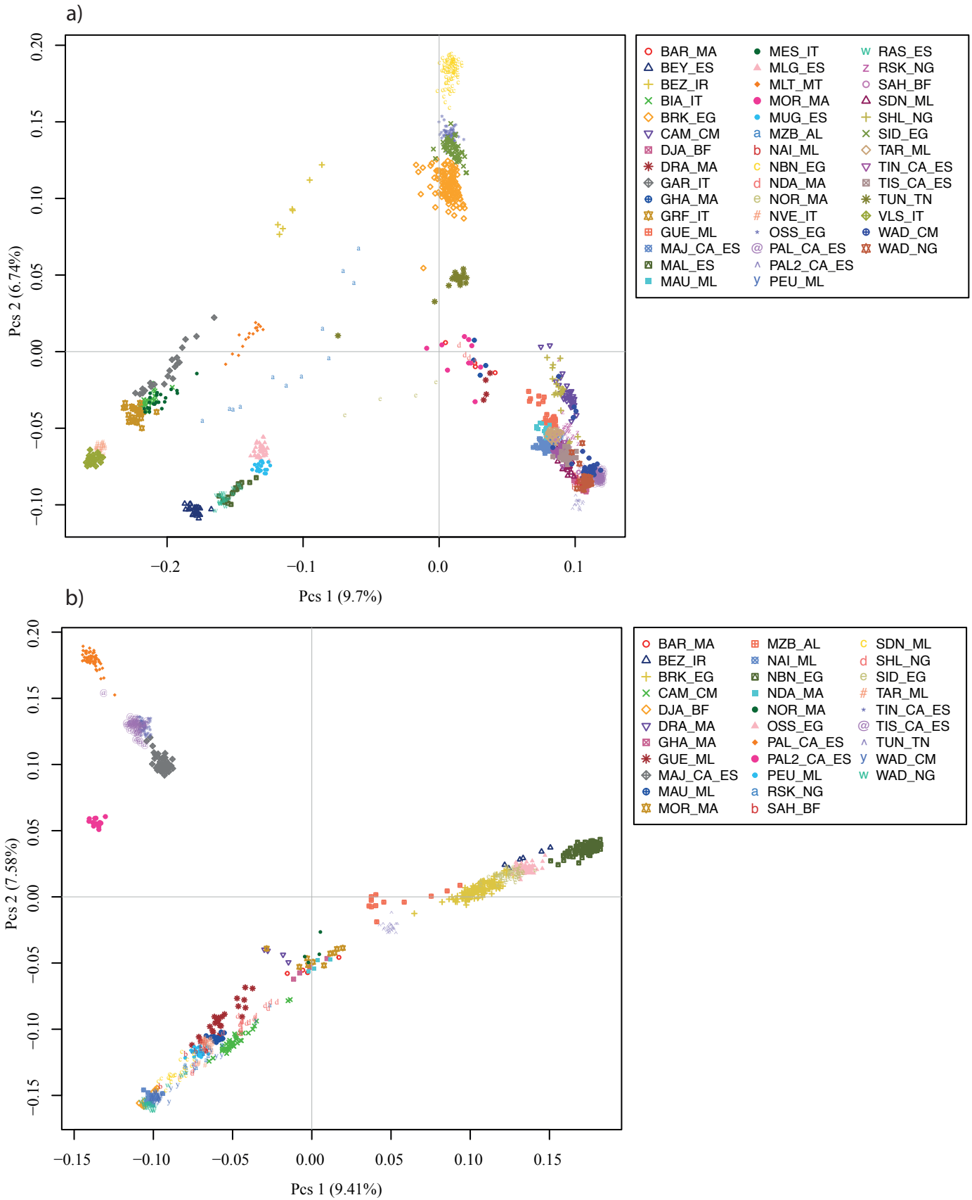
Figure S3. The Multidimensional Scaling Plot (MDS) of the analyzed breeds using the whole dataset a) and the AFR-CAN dataset b). See Table 1 for more details.
