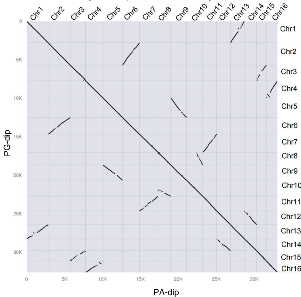
Inter-genomic comparison: PA vs. PG (30,536 gene pairs)
