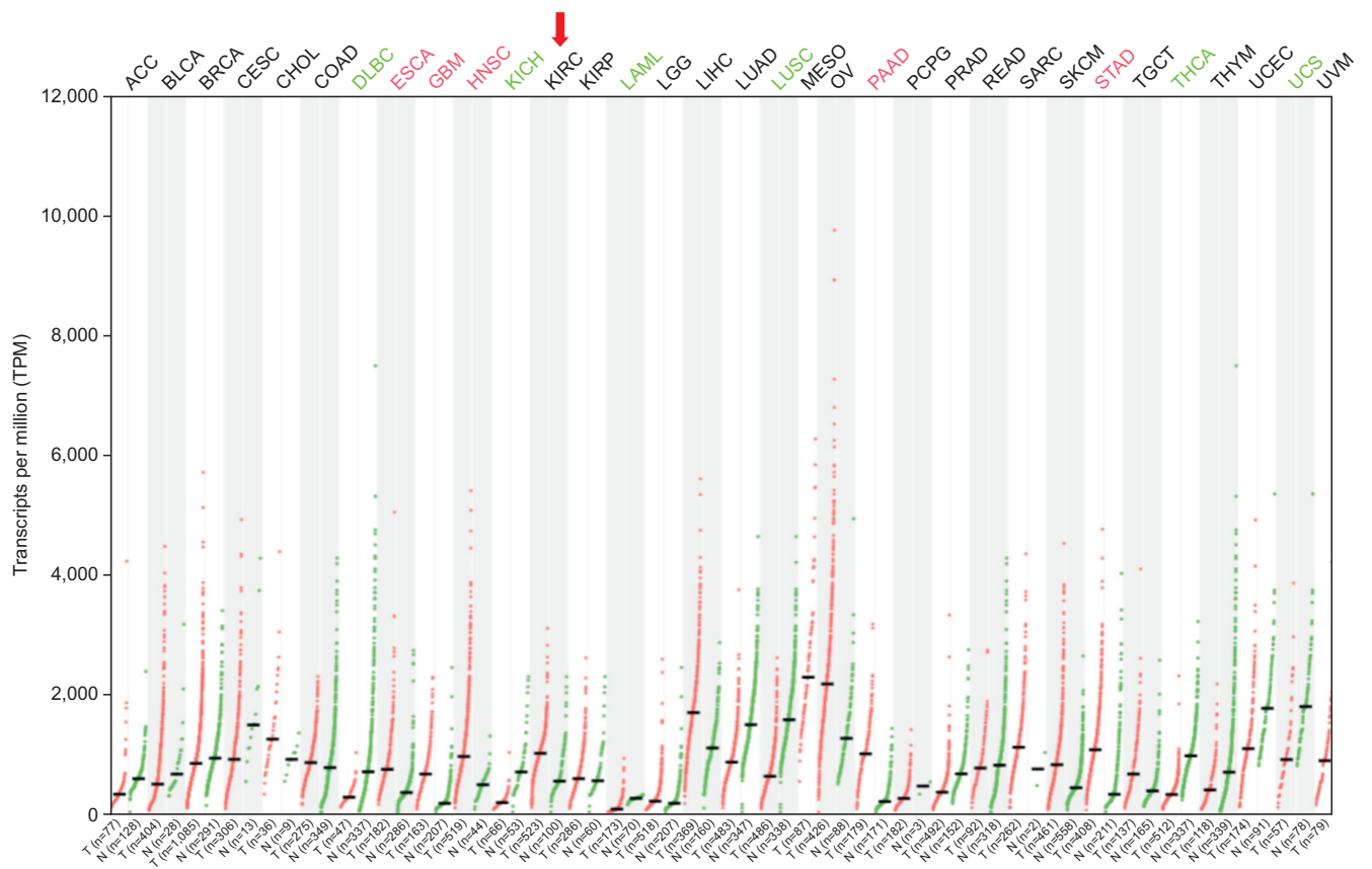
Supplementary Fig. 2. Increased expression of IFITM3 (interferon-induced transmembrane protein 3) in renal cell carcinoma (RCC) compared to the normal kidney in a public database GEPIA.
