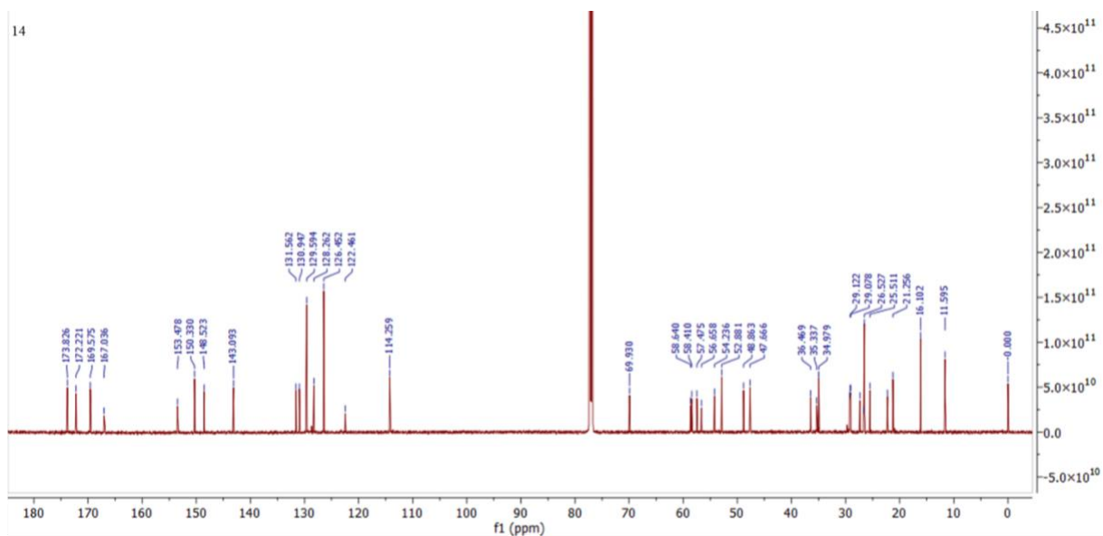
1 H NMR spectrum of compound 27
