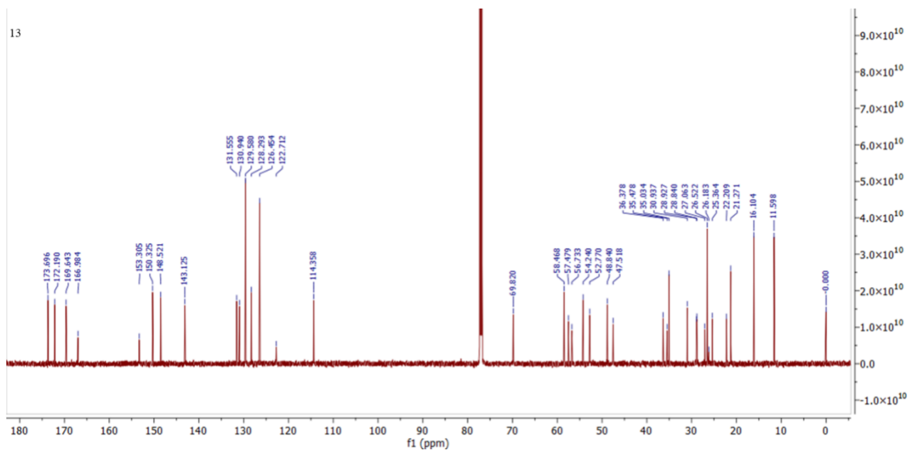
^1\text{H} NMR and ^{13}\text{C} NMR spectrum of YX968-NC
