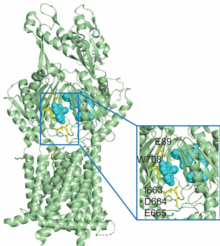
Figure S1. Structure of the ligand-bound AdeB protomer. Three Et molecules bound to AdeB are shown as cyan spheres. The insert shows the mutated amino acid residues E89, W708, I663, D664, E665.
