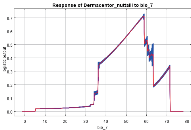
Temperature Annual Range
