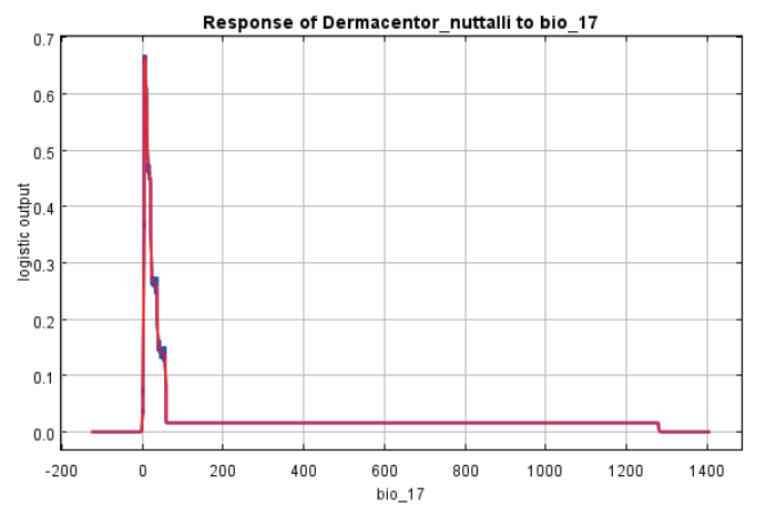
Precipitation of Driest Quarter
