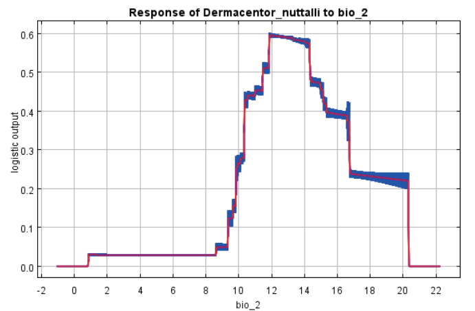
Mean Diurnal Range
