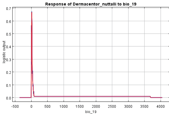
Precipitation of Coldest Quarter
