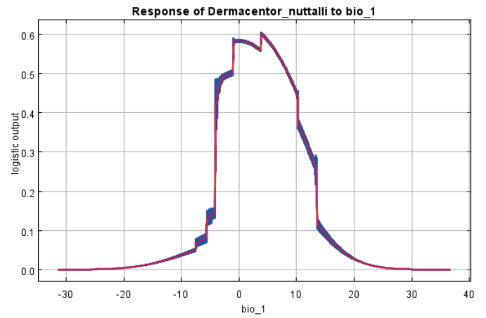
Annual Mean Temperature
