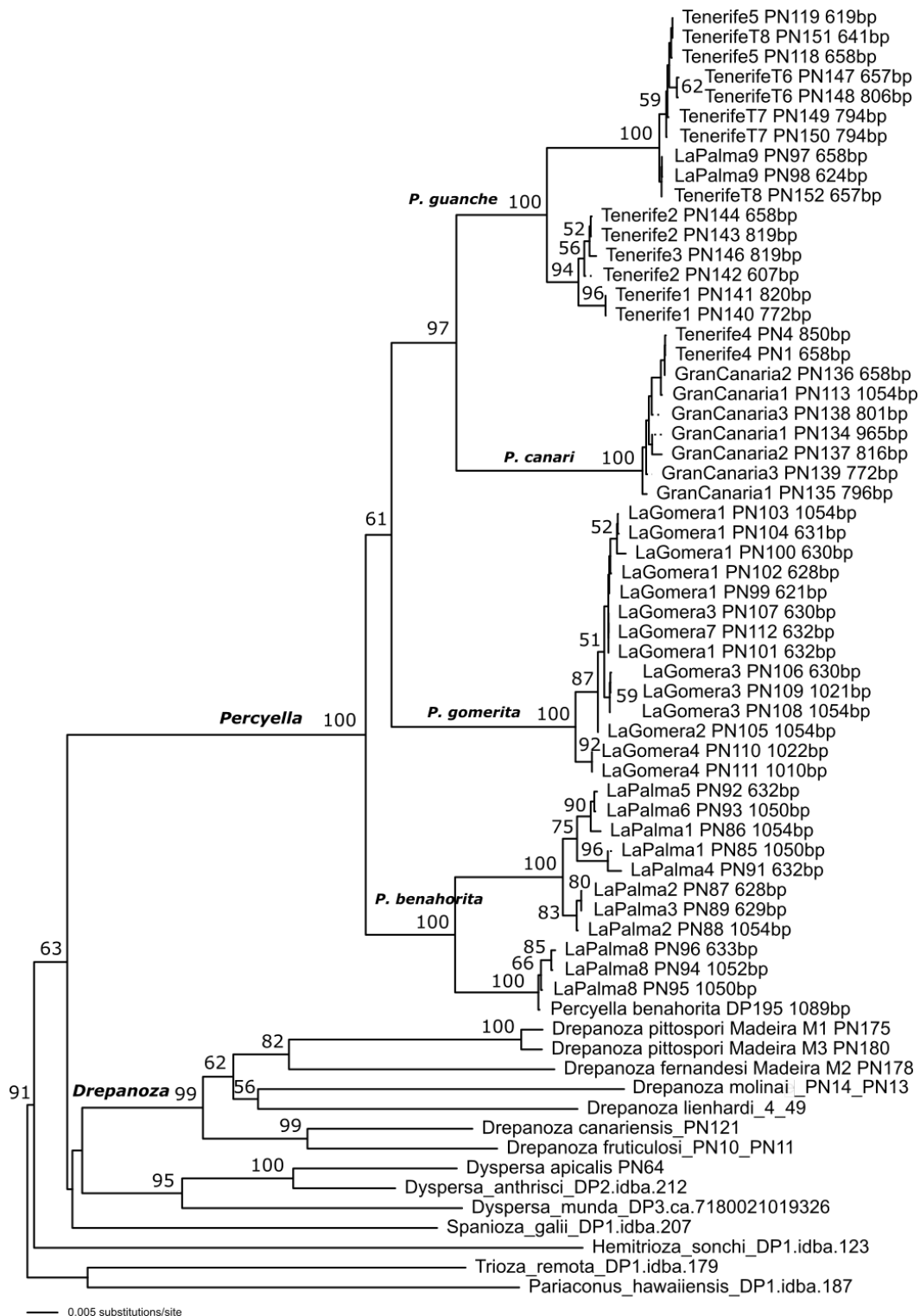
Figure S1. Neighbor-joining analysis using cox1 data for Percyella , Drepanoza , and select outgroup taxa from Group A (Percy et al. 2018) [52]. Full length sequences were used for the Percyella samples (sequence length shown with sample code).
