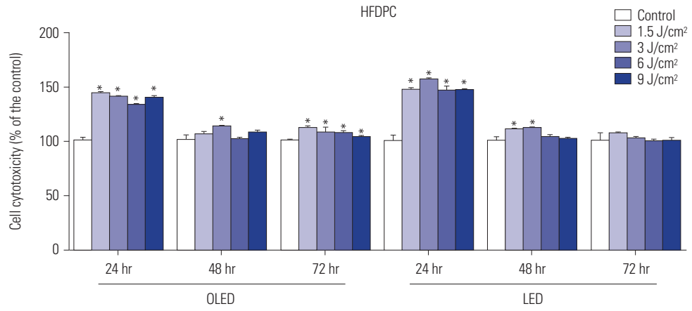
Supplementary Fig. 3. Safety assessment of OLED and LED light irradiation on HFDPCs were performed via confirmation of cell viability. * p < 0.05 , independent samples t-test. HFDPCs, hair follicle dermal papilla cells; LED, light-emitting diode; OLED, organic light-emitting diode.
