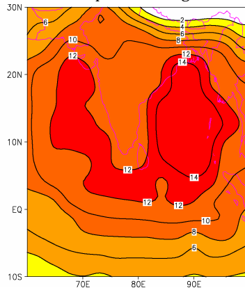
C) Atmospheric forcing
