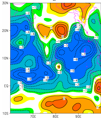
A) TOA forcing
