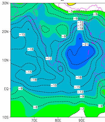
B) Surface forcing
