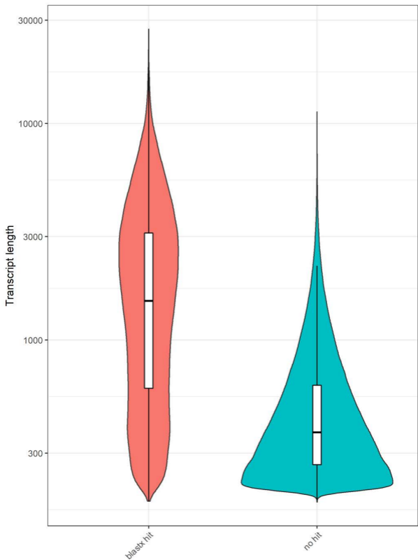
Suppl. Figure 1 : Transcript lengths. Distribution of transcript lengths for transcripts that had a significant blastx hit against the mouse proteome and those that did not. The width of each violin indicates the number of transcripts at the respective size range. The boxes show the median transcript length (center line) and the 25th and 75th percentiles (upper and lower edges of the boxes, respectively).
