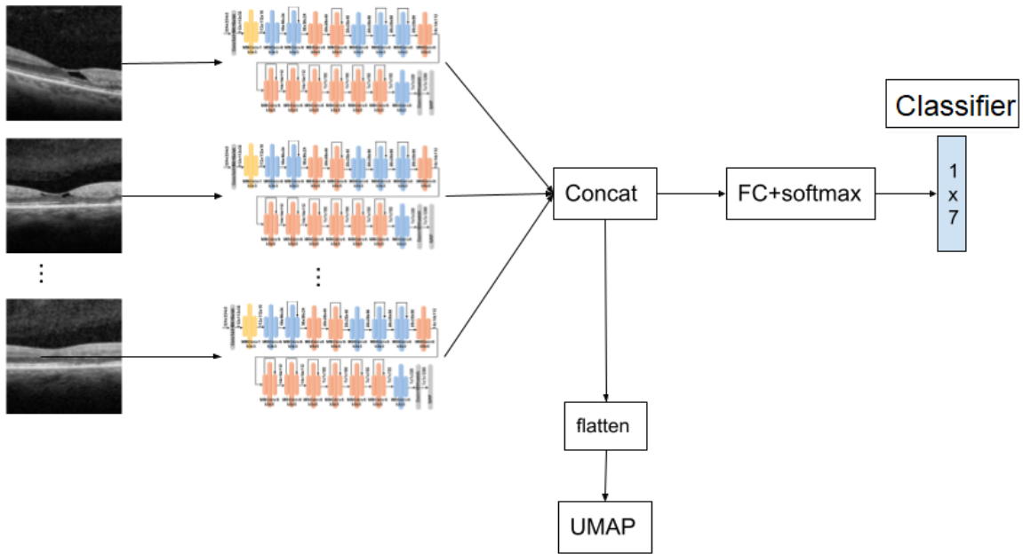
Supplemental Figure 3. Schematic of Multi-view classifier and extraction of its last feature layer to learn a UMAP embedding. 20 central B-scans are given as input to a EfficientNet-B0 classifier, and the last layer of trained classifier is extracted as input for the UMAP.
